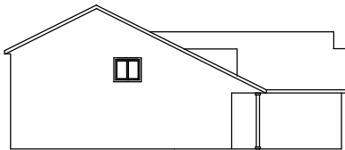
LEFT ELEVATION
